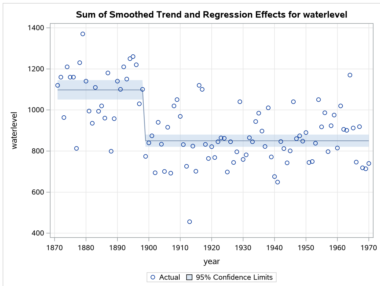
Output 42.7.4 Smoothed Trend plus Shift of 1899
