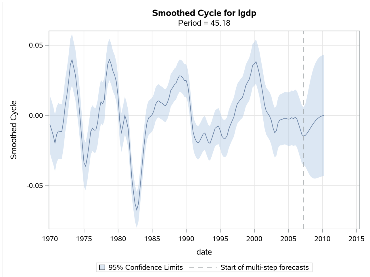
Output 42.9.3 Estimated Cycle: Order = 2
