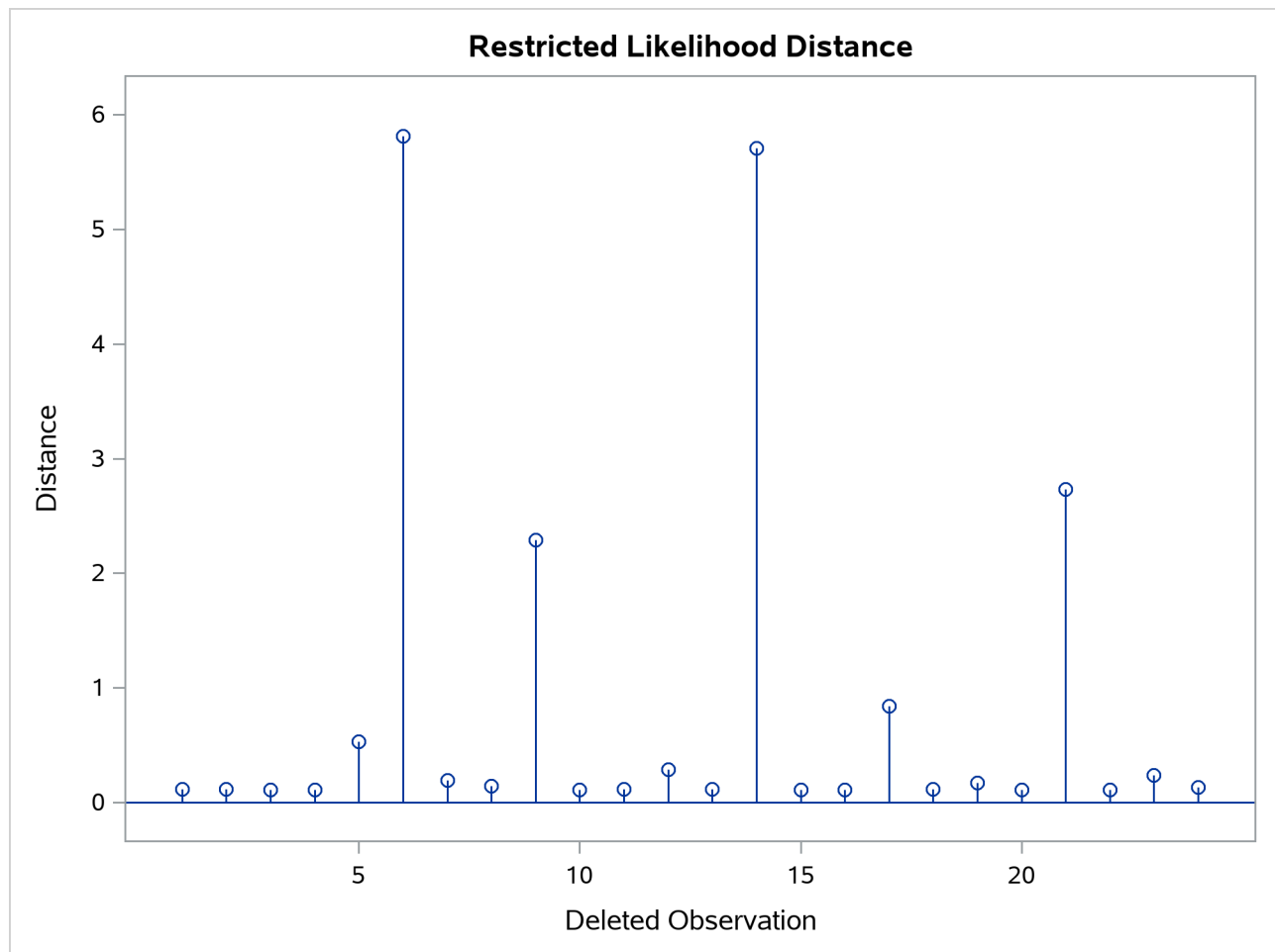
Output 81.7.7 Restricted Likelihood Distance
