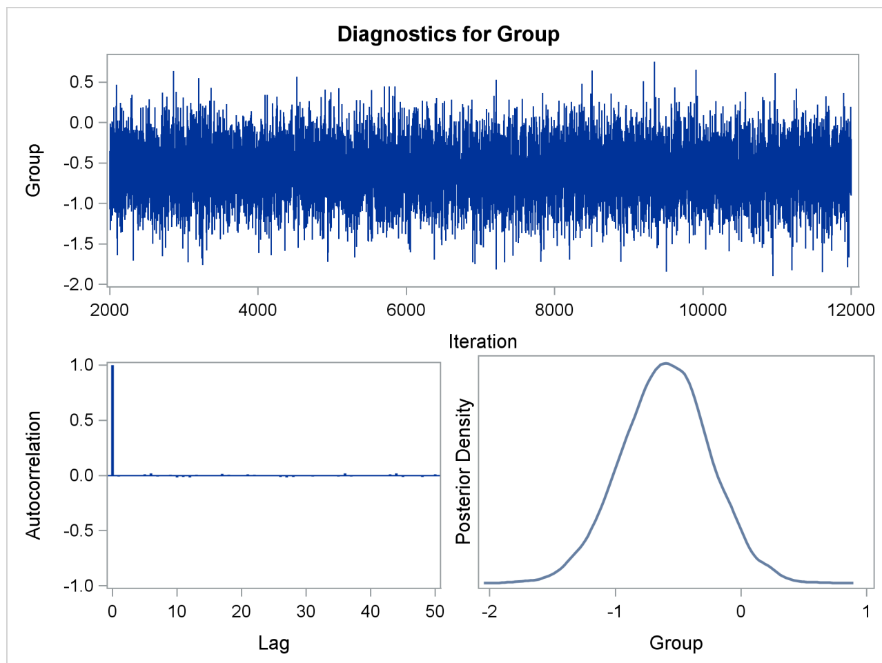
Figure 87.10 Diagnostic Plots
