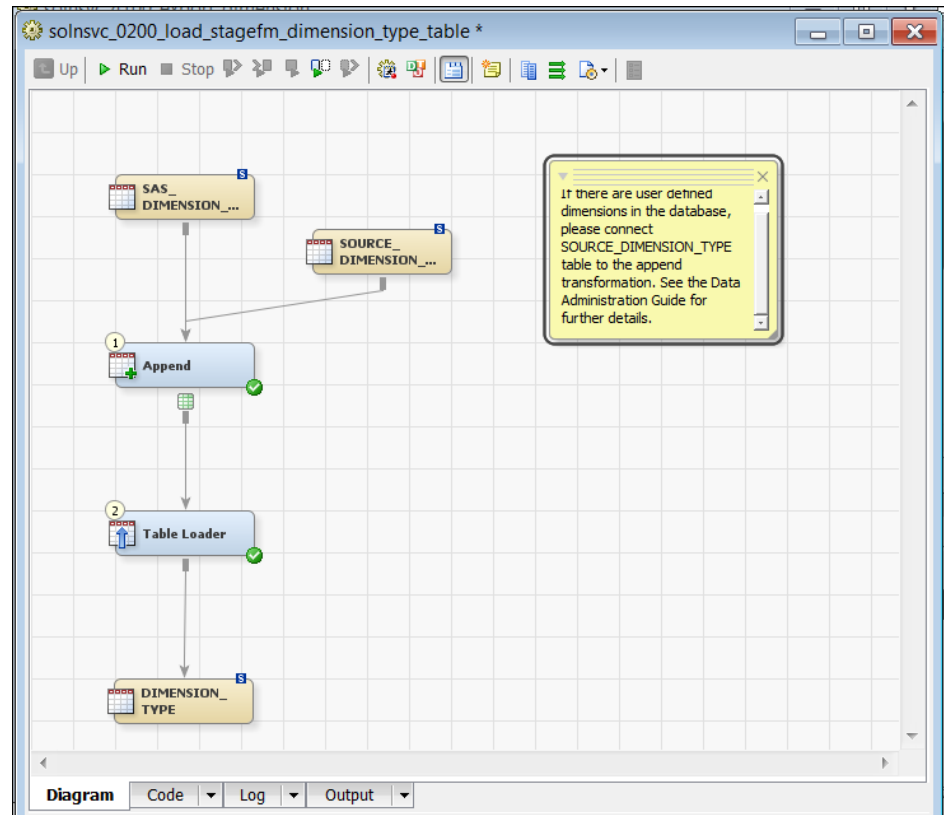
Figure 10.3 solnsvc_0200_load_stagefm_dimension_type_table Process Diagram
