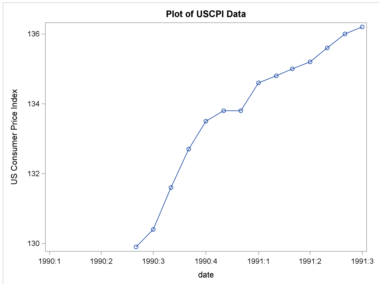
Figure 3.9 Plot of Monthly CPI over Time
