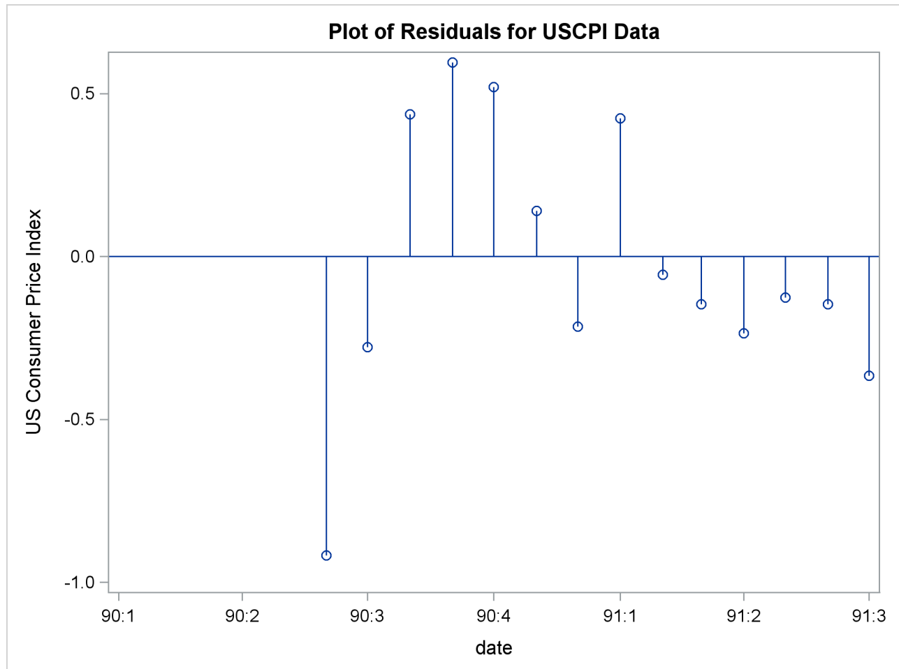
Figure 3.12 Plot of Residuals
