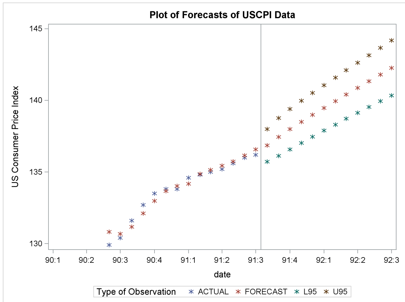
Figure 3.11 Plot of Forecast
