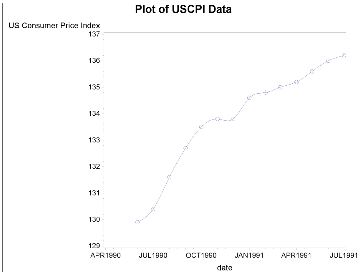
Figure 3.13 Plot of Monthly CPI over Time
