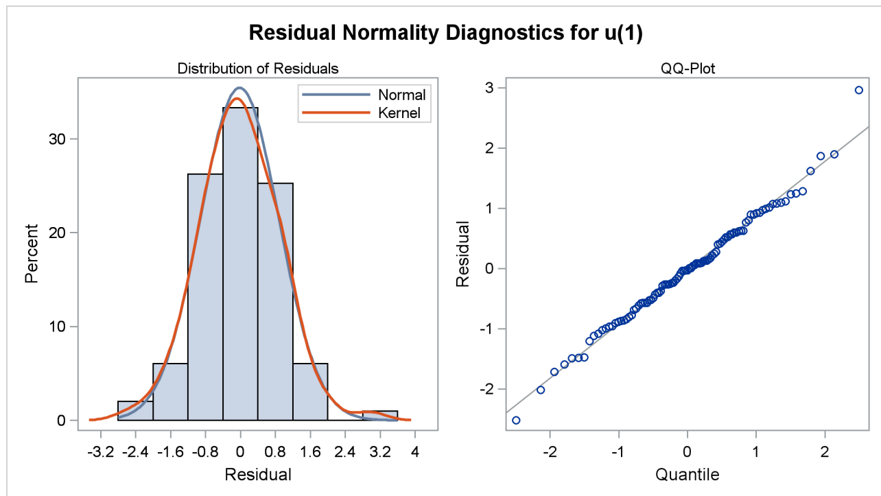
Output 7.1.5 Residual Normality Analysis of the ARIMA(0,1,1) Model
