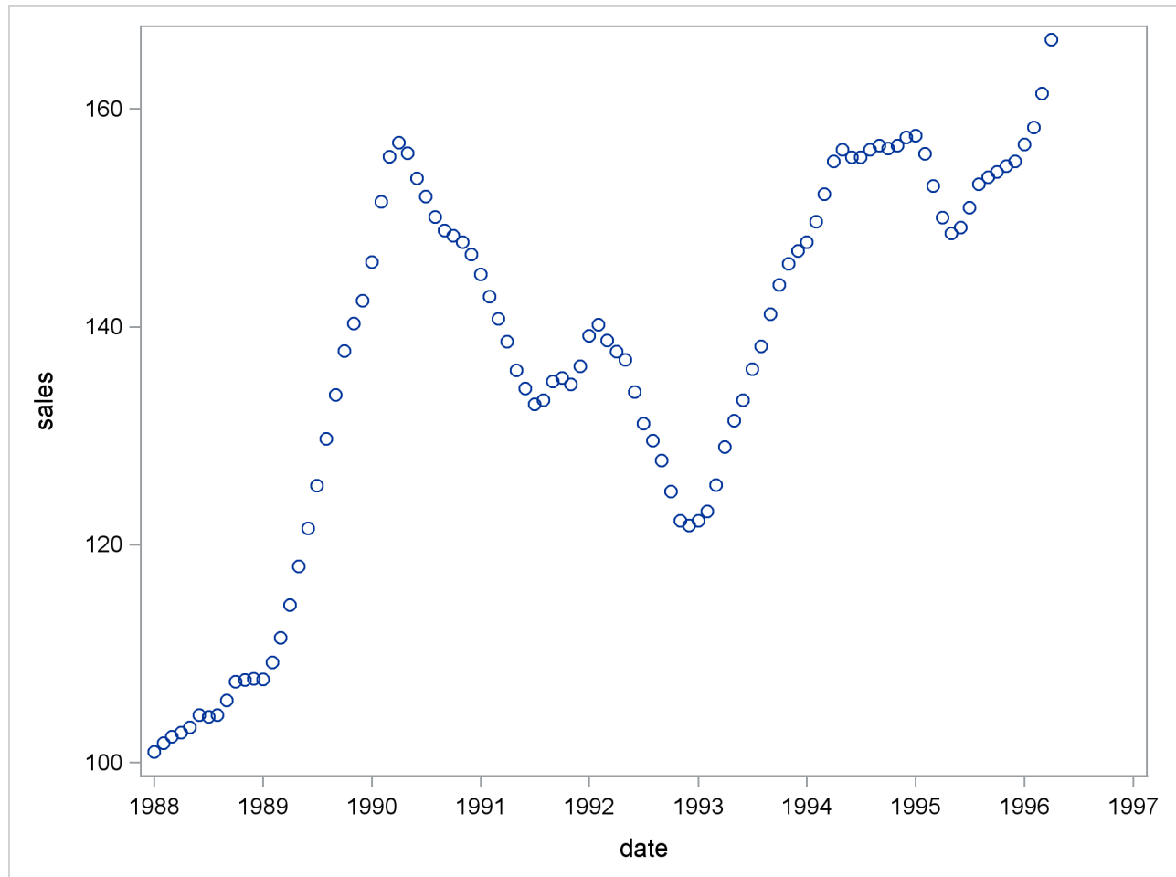
Figure 7.1 Simulated ARIMA(1,1,1) Series SALES
