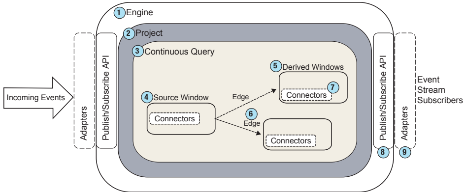
The Event Stream Processing Model Hierarchy
