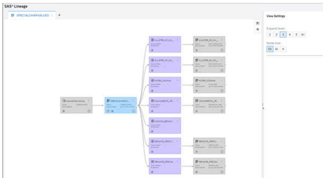
Figure 6 Expansion Level 3
