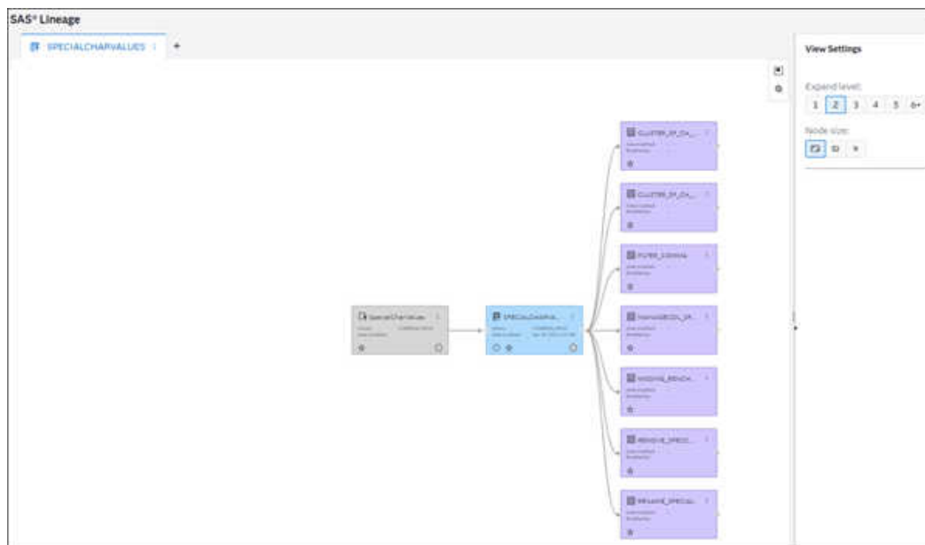
Figure 5 Expansion Level 2
