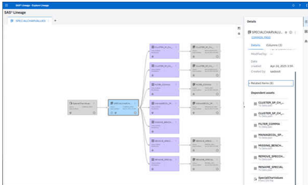
Figure 1 Analysis Flow
